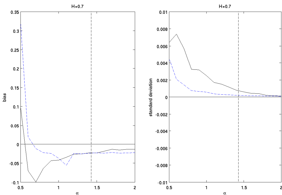
FIGURE 2. Bias and standard deviations of the FIRT estimators \hat{H}_{FIRT} - H (solid line) and the wavelet estimators \hat{H}_{WT} (dashed line) studied in [16] as functions of \alpha when H = 0.7 . The broken vertical line located at \alpha = 1/H indicates on the right the long range dependence cases. The bias and standard deviations were computed by using samples of n = 256 independent replications of the estimators, obtained from 256 independently simulated paths of the LFSM process for N = M = 2^{16} points, L = 2^{18} and A = 101 .
