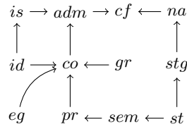
Fig. 3: Extension Inclusion Graph Inc(\mathcal{S})
