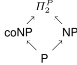
Fig. 2: Complexity Graph Comp(\mathcal{S}, T)
