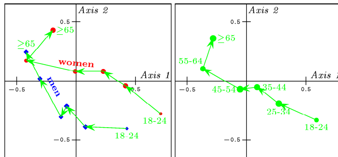
Figure 4.7 Taste example. Five successive within-effects (vectors) of Age for each gender (left) and main effects (vectors) of Age (right) in plane 1-2.
