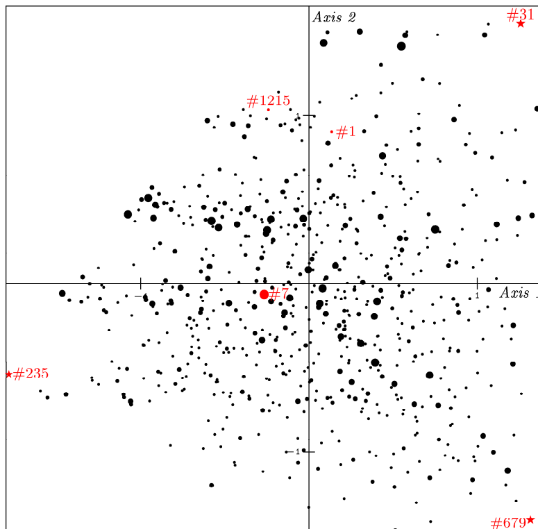
Figure 1.3 Cloud of 1215 individuals with landmark individuals (*) in principal plane 1-2.
