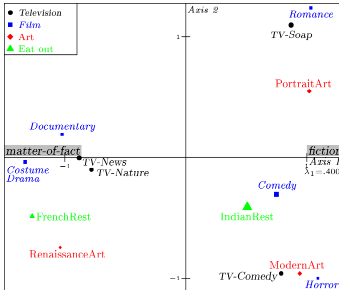
Figure 3.5 Taste Example. The 14 categories selected for the interpretation of Axis 1 in plane 1-2.
