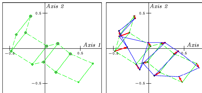
Figure 4.8 Additive cloud fitted to the Gender x Age cloud (left) and the 12 deviations (vectors) from the Gender x Age cloud (right).
