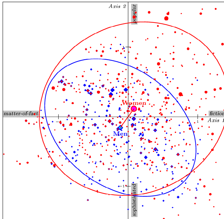
Figure 4.2 Taste Example. Subclouds of men and women in principal plane 1-2 with mean points and concentration ellipses.
