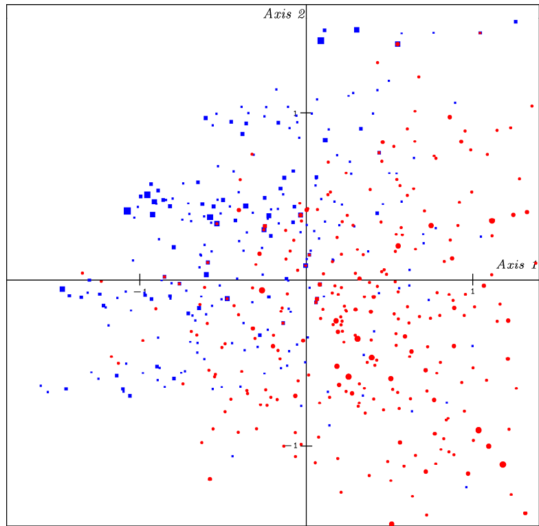
Figure 1.4 Taste Example. Two subclouds of individuals corresponding to over 55 and 18-34 age groups, in principal plane 1-2.
