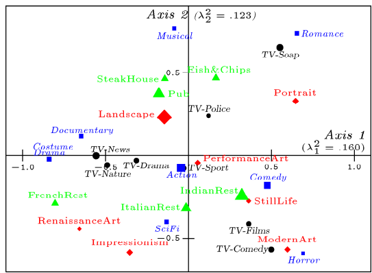
Figure 3.11 Taste Example. Burt cloud of the 29 category mean points in principal plane 1-2 (cloud of individuals). The scale is the same as the one of the cloud of categories (Figure 1.2, p.7).
