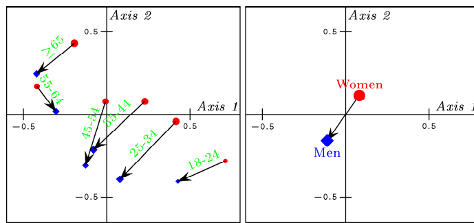
Figure 4.6 Taste example. Six within-effects (vectors) of Gender for each age group (left) and main effect (vector) of Gender (right) in plane 1-2.
