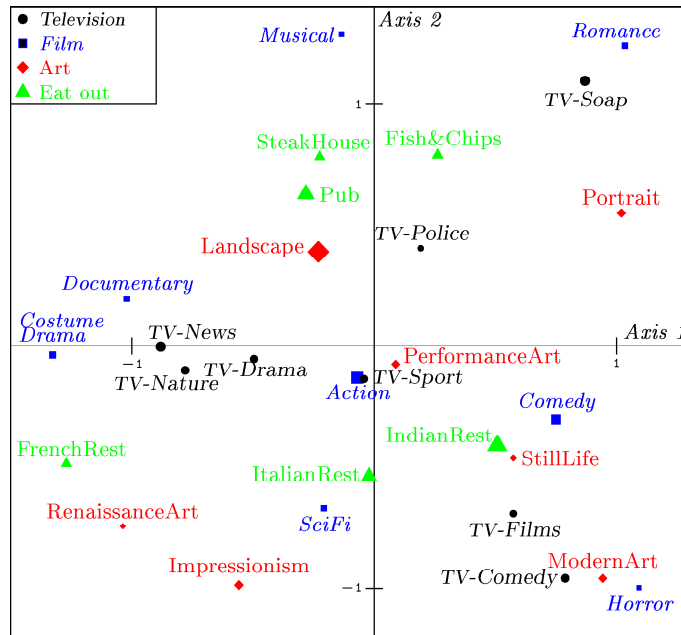
Figure 1.2 Taste Example. Cloud of the 29 categories of the four questions in principal plane 1-2.
