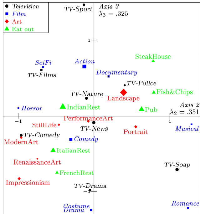
Figure 3.1 Taste Example . Principal cloud of the 29 categories in plane 2-3.
