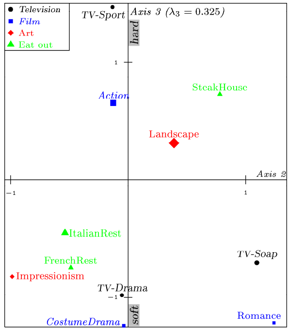
Figure 3.7 Taste Example. The 11 categories selected for the interpretation of Axis 3 in plane 2-3.
