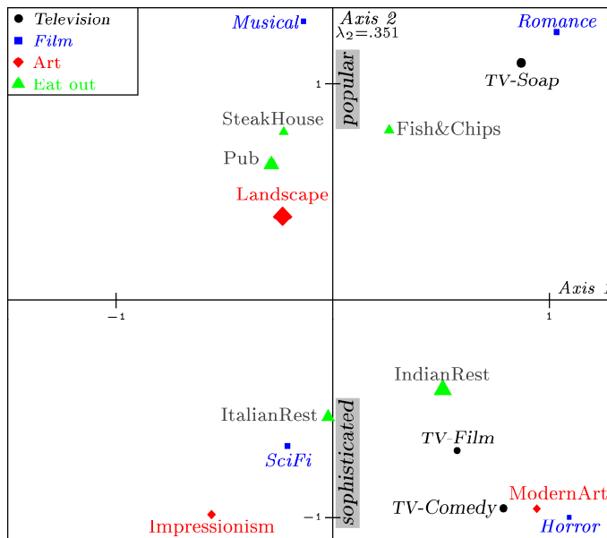
Figure 3.6 Taste Example. The 15 categories selected for interpretation of Axis 2 in plane 1-2.
