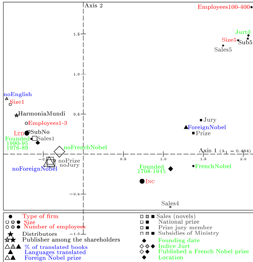
Figure 6.1 Plane 1-2: 25 categories selected for interpreting Axis 1.
