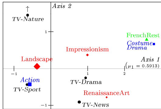
Figure 3.12 Taste Example. Cloud of the 10 categories selected for the interpretation of specific Axis 1, in specific plane 1-2 (half size). (The coordinate of TV-Nature relative to Axis 2 is equal to 2.75, hence the arrow).
