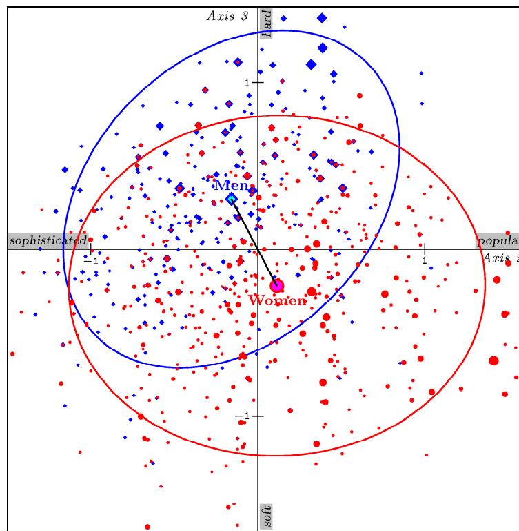
Figure 4.3 Taste Example. Subclouds of men and women in principal plane 2-3 with mean points and concentration ellipses.
