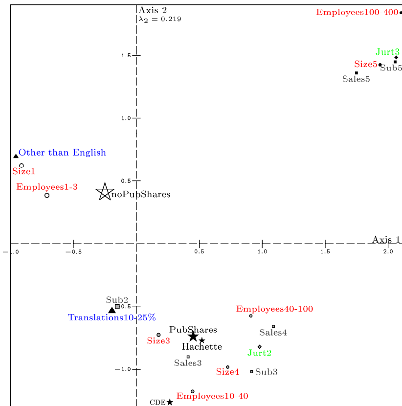
Figure 6.3 Plane 1-2: 22 categories selected for interpreting Axis 2.
