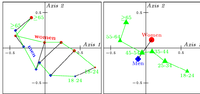
Figure 4.5 Taste Example. Age x Gender cloud (left), Gender and Age clouds (right) in plane 1-2 (same scale as Figure 1.3, p.8).
