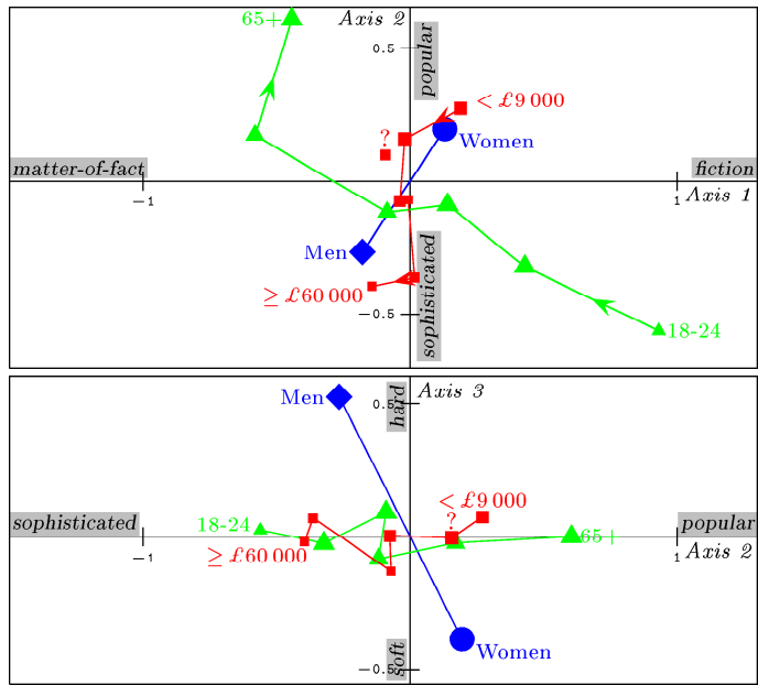
Figure 3.9 Taste Example. Supplementary questions in plane 1-2 (top), and in plane 2-3 (bottom) (cloud of categories).
