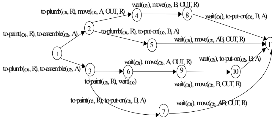
Figure 1: The negotiation graph
